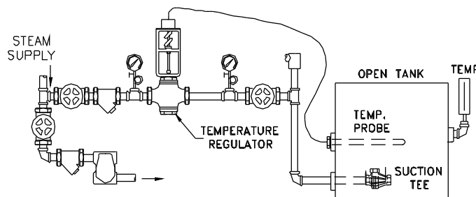
CONTROLLING TEMPERATURE OF LARGE OPEN TANK BY STEAM INJECTION
