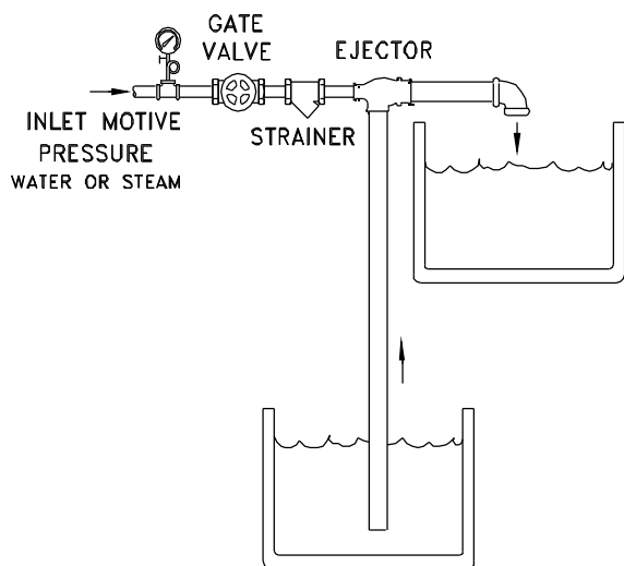
EJECTOR LIFTING LIQUID
