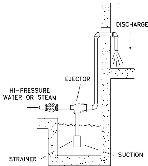
LIFTING WATER TO A HIGHER LEVEL WITH WATER OR STEAM PRESSURE
